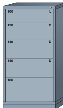
5 drawers with 37 compartments
