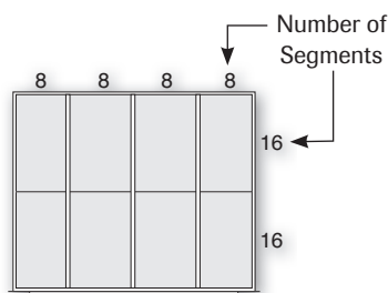
Sample Layout for 70 Drawer Dividers = (4) 24067D8
