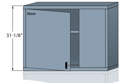
Base shelf and adjustable shelf behind lockable swing doors without base channels ■ ■ 251350X1055
